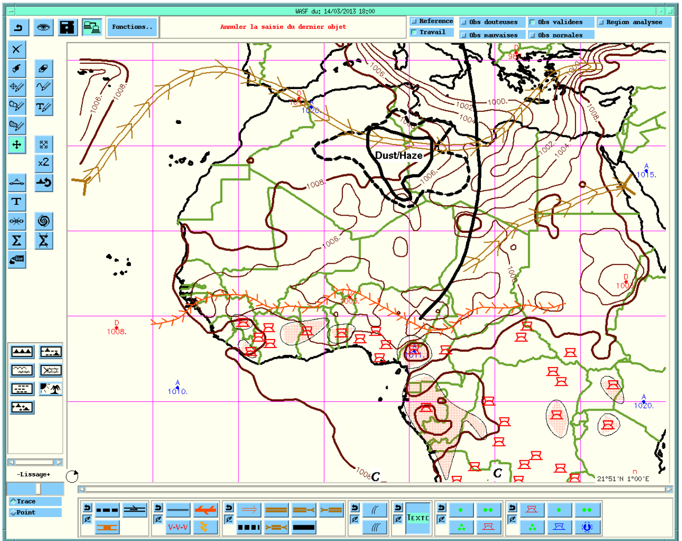
Figure 2: WASA for 14/03/2013 at 1800Z
