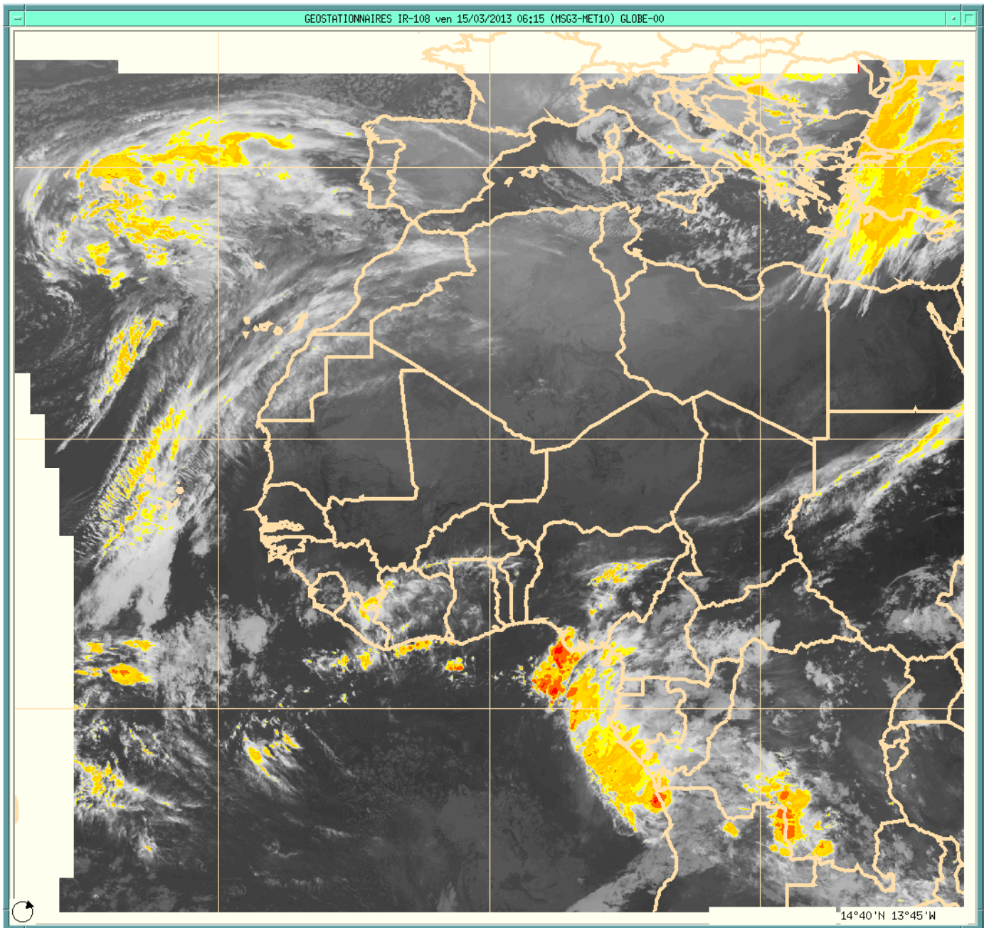
Figure 3: SAT PIC 0615 UTC ON 15/03/2013
