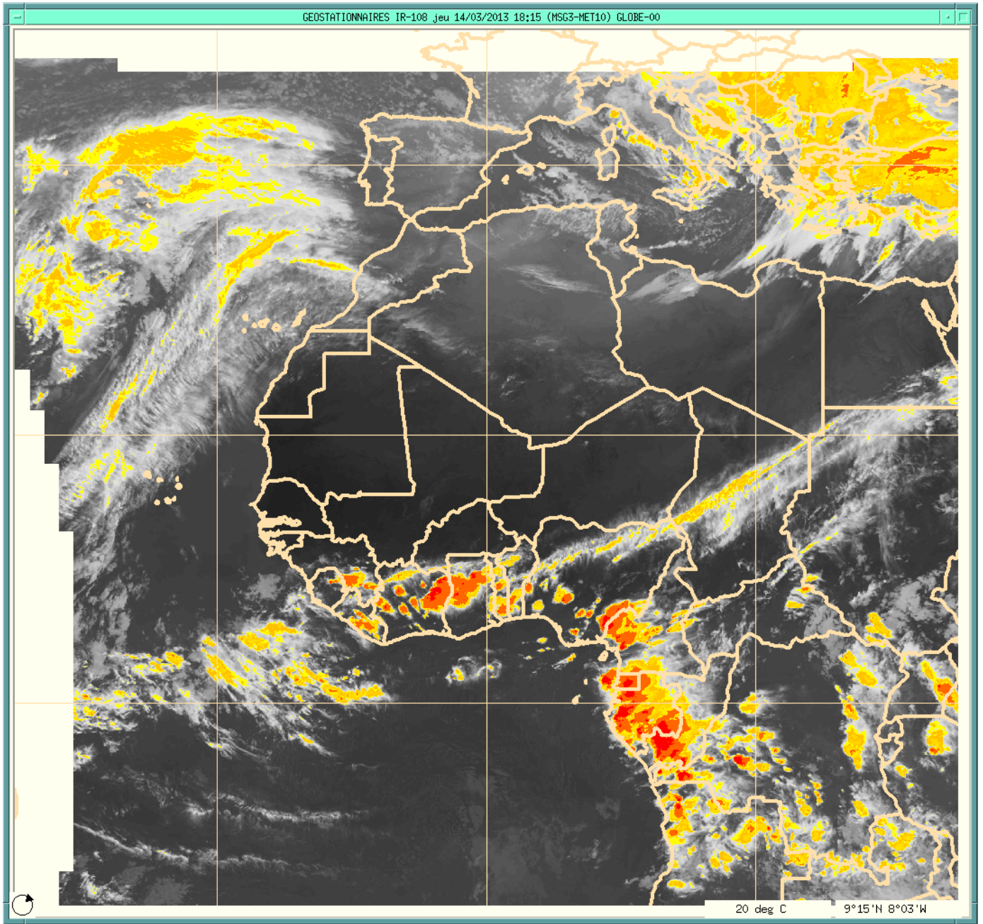
Figure 1: SAT PIC 1815 UTC ON 14/03/2013
