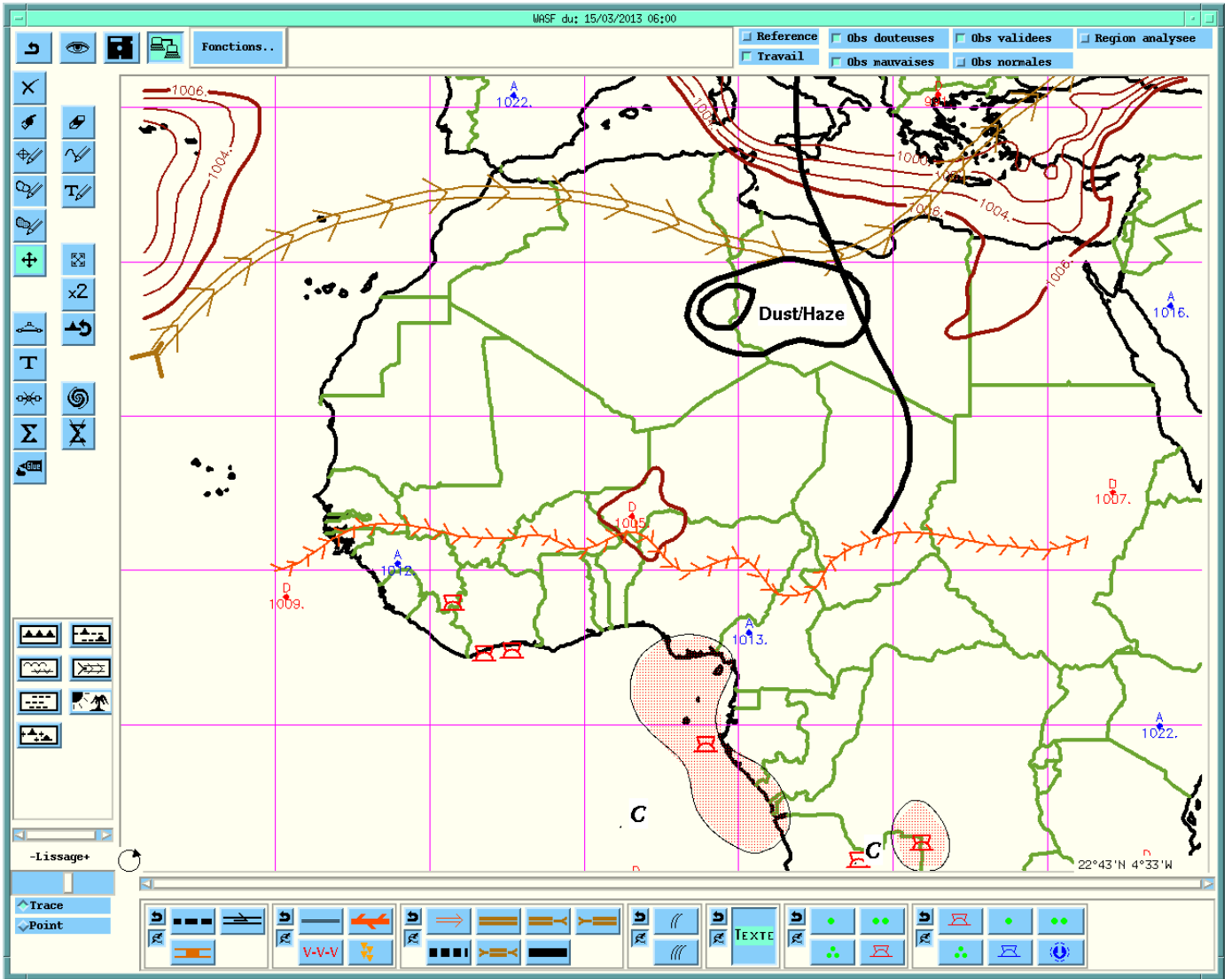
Figure 4: WASA for 15/03/2013 at 0600Z
