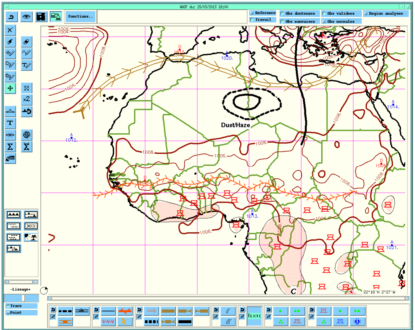
Figure 5: WASF for 15/03/2013 at 1800Z
