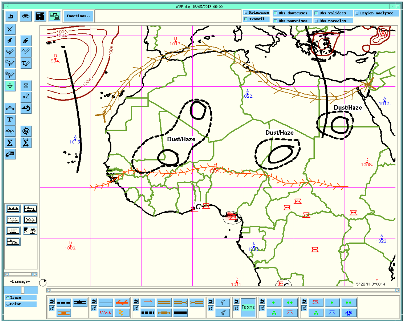
Figure 6: WASF for 16/03/2013 at 0600Z
